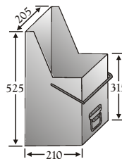
Fuel Carrier Part No. 01429
