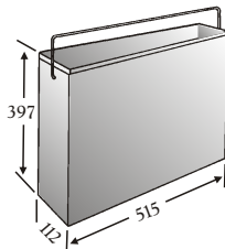
Multi-Fuel Ash Container Part No. 01414
